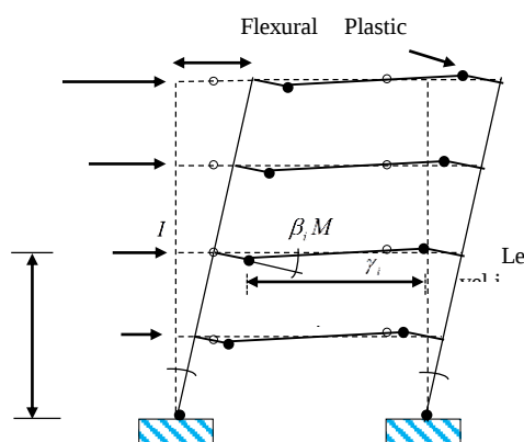
Figure 1. Single-bay frame prototype with predefined mechanism and plastic hinges in beams and column end
