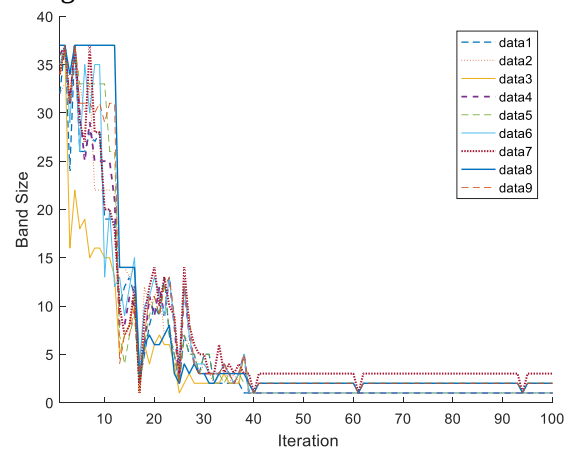
Figure 11. BS variation up to iteration 100 for the design variables in 1512-bar truss design
